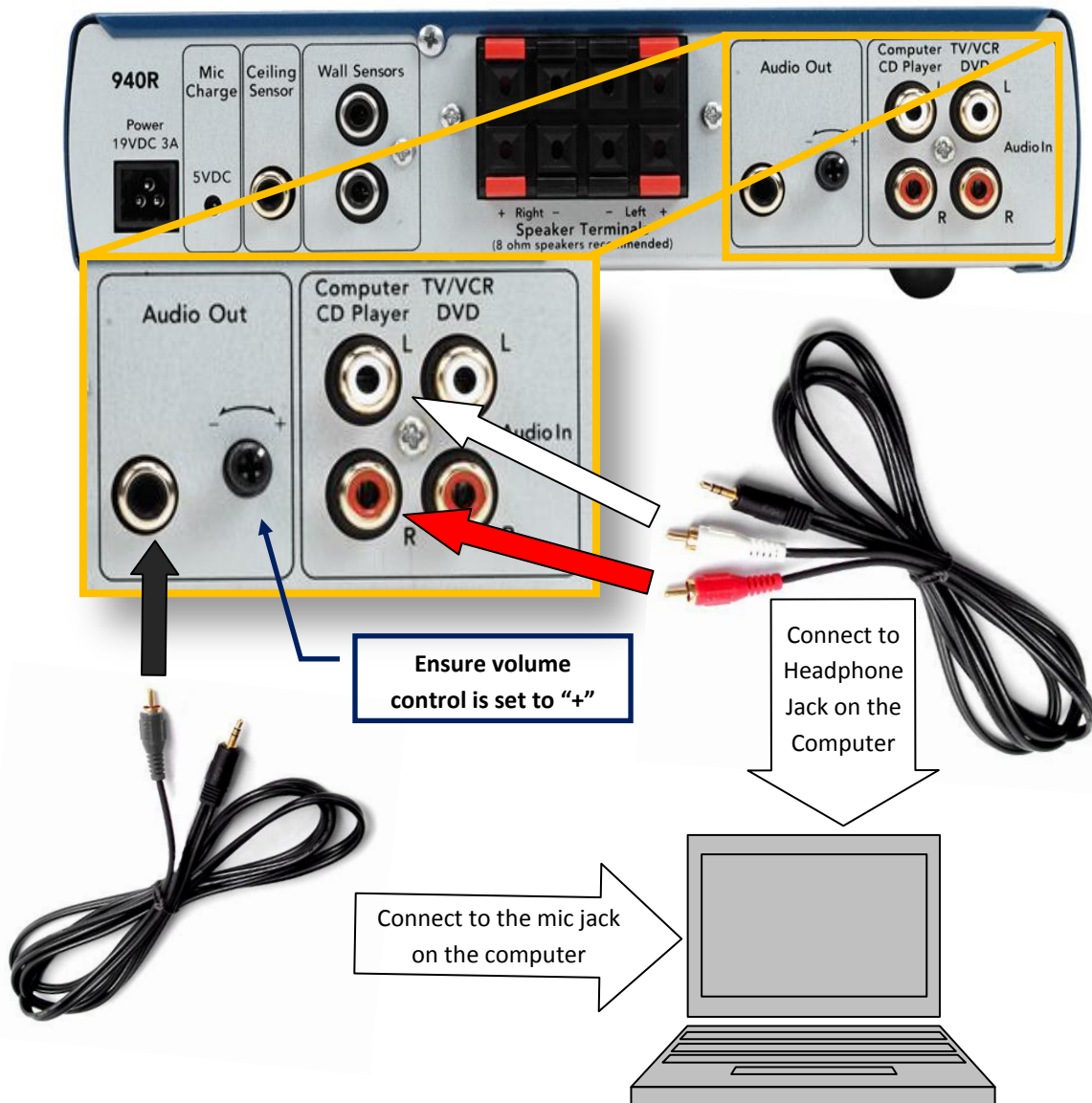
Back of 940R Receiver
